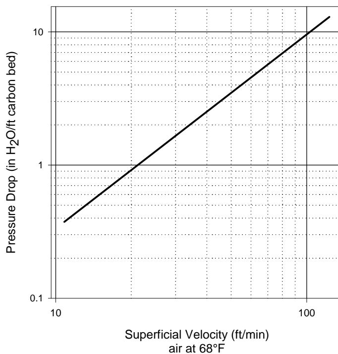
Typical Pressure Drop Curve for NORIT VAPURE 612
