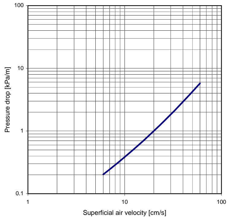
Typical Pressure Drop Curve for 4 mm Extruded Pellets
