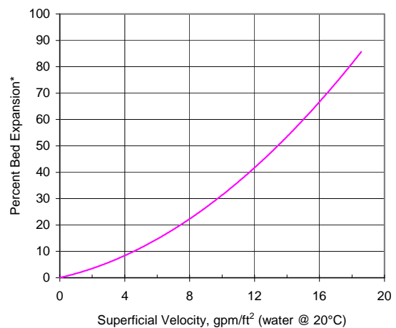
Bed Expansion Curve for HYDRODARCO 3000
