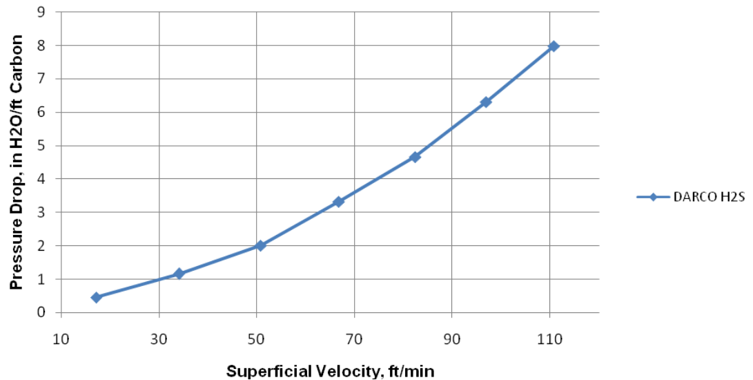
Typical Pressure Drop Curve
