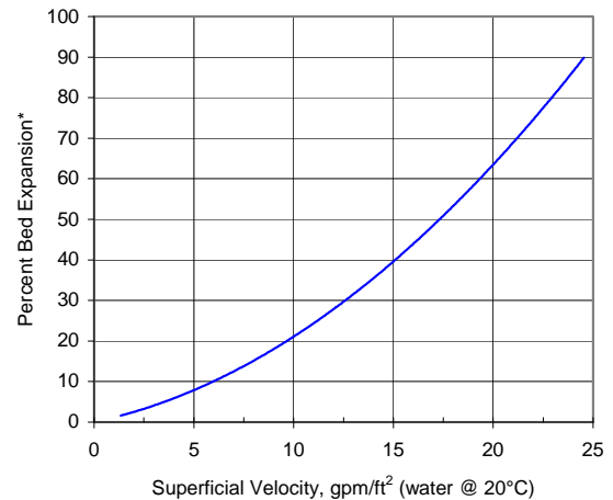
Bed Expansion Curve for NORIT GAC 840R
