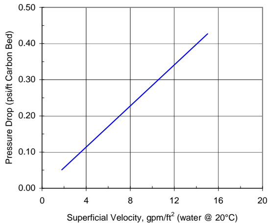
Pressure Drop Curve for NORIT GAC 840R
