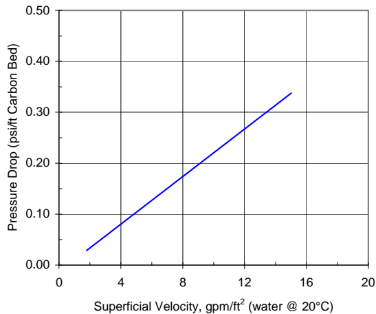
Pressure Drop Curve for NORIT GAC 830
