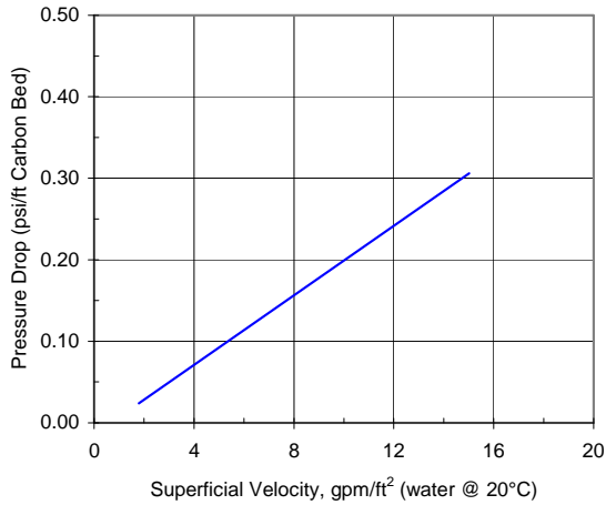
Pressure Drop Curve for NORIT GAC 830 PLUS
