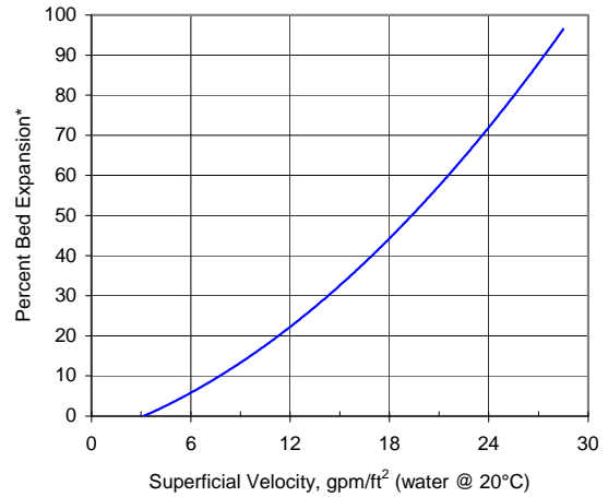
Bed Expansion Curve for NORIT GAC 830 PLUS
