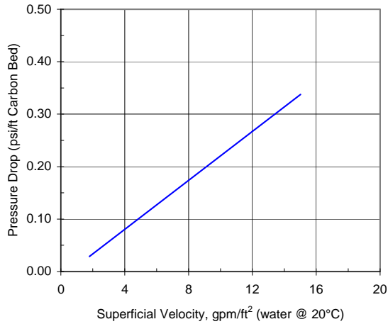
Pressure Drop Curve for NORIT GAC 300
