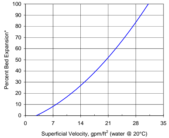
Bed Expansion Curve for NORIT GAC 300
