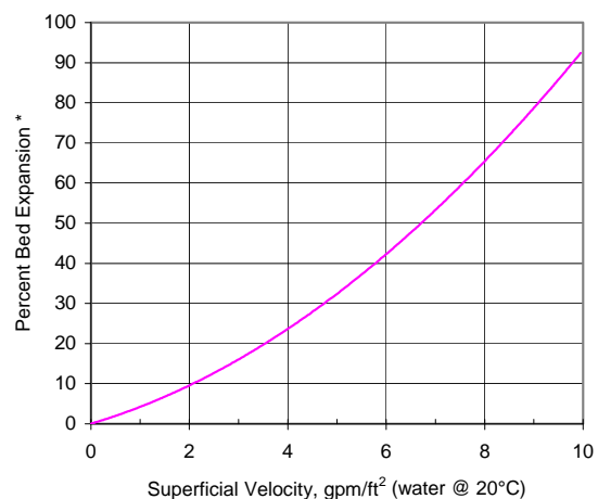
Bed Expansion Curve for DARCO 20X40
