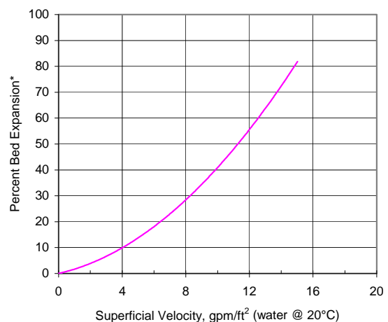
Bed Expansion Curve for DARCO 12X40
